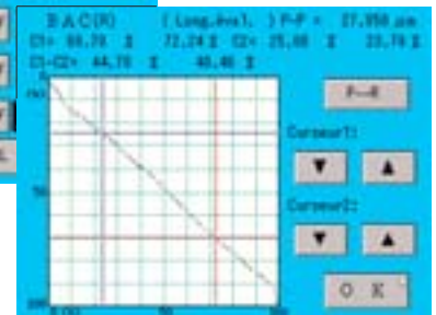
Material ratio curve (BAC)
